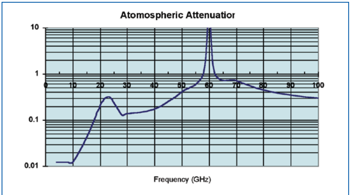
Figure 3: Atmospheric Attenuation as a Function of Frequency
