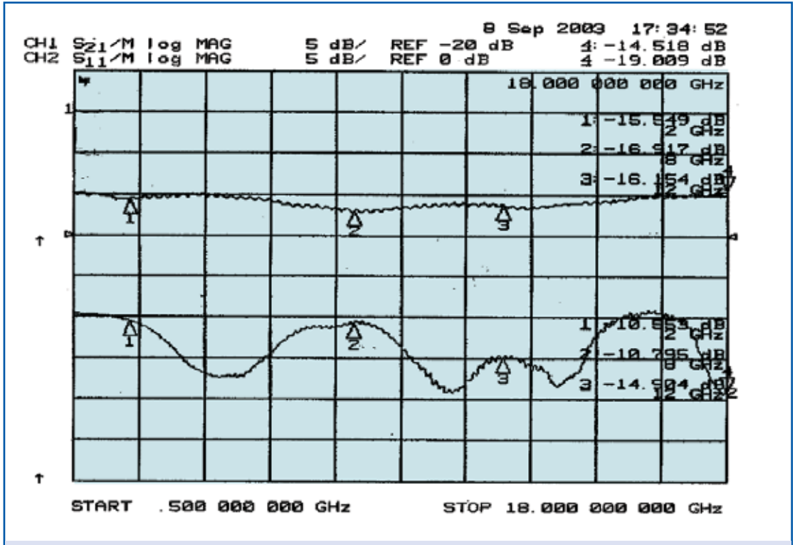
Figure 2: 13 Meter MilTech( 340 Cable Assembly With Equalized Low Noise Amp Incorporated
